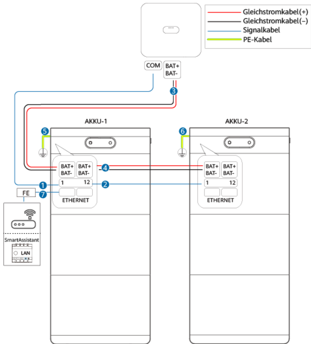
Abbildung 5-1 ESS-Kabelanschlüsse
